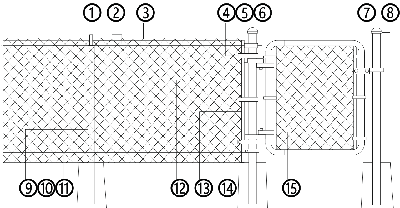
Fittings for chain link fence assembled with gate
